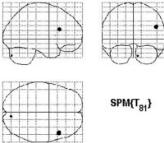
Figure 1: CBF increase in subtraction condition "2 - 2C"
